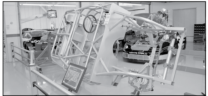
Cut aways show how the cars are built
